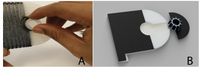
Figure 7: a) Shows the rotary encoders fabricated with FiberWire. The casing includes partially filled carbon fiber in semi-circle and the knob fully filled with carbon fiber b) Shows the assembly of the encoder
