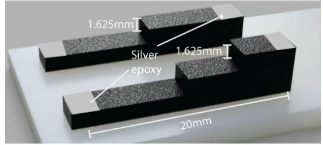
Figure 4: Resistance characterization test between layers
