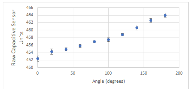
Figure 8: Shows the characterization of capacitance vs angle of our rotary encoder design
